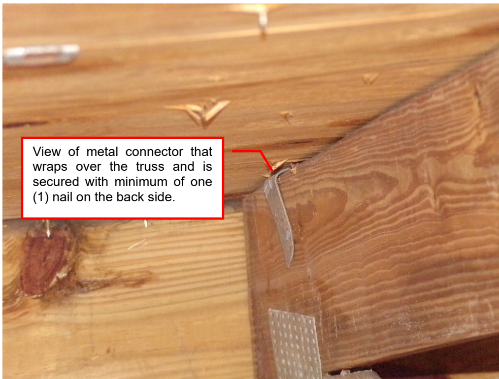
View of metal connector used on Roof to Wall attachment (per question 4).
