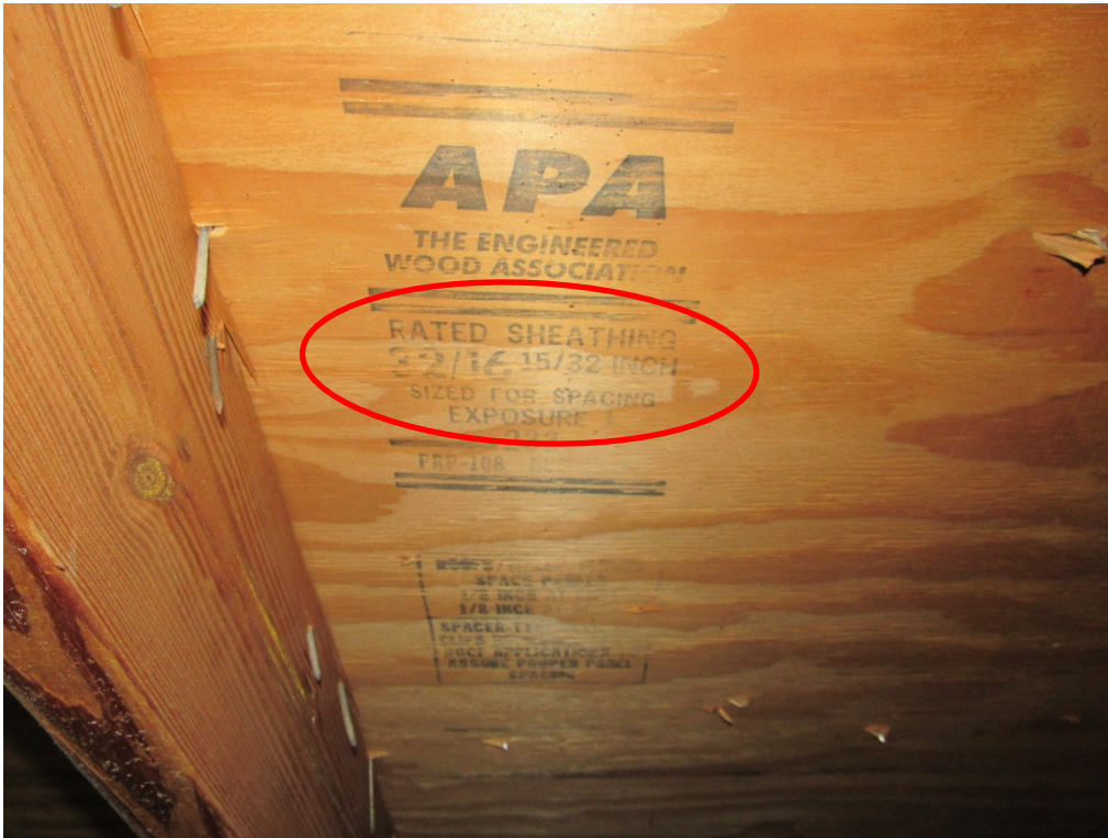
View of existing plywood sheathing thickness (15/32) per question 3.
