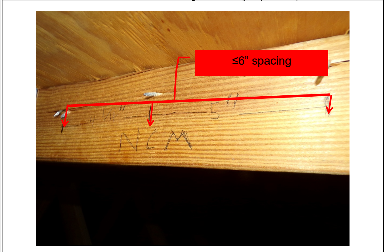
View of re-nailing pattern (per question 3).
