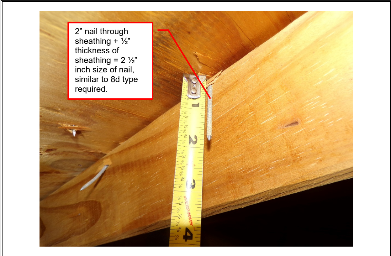
View of nail used on sheathing attachment (per question 3).
